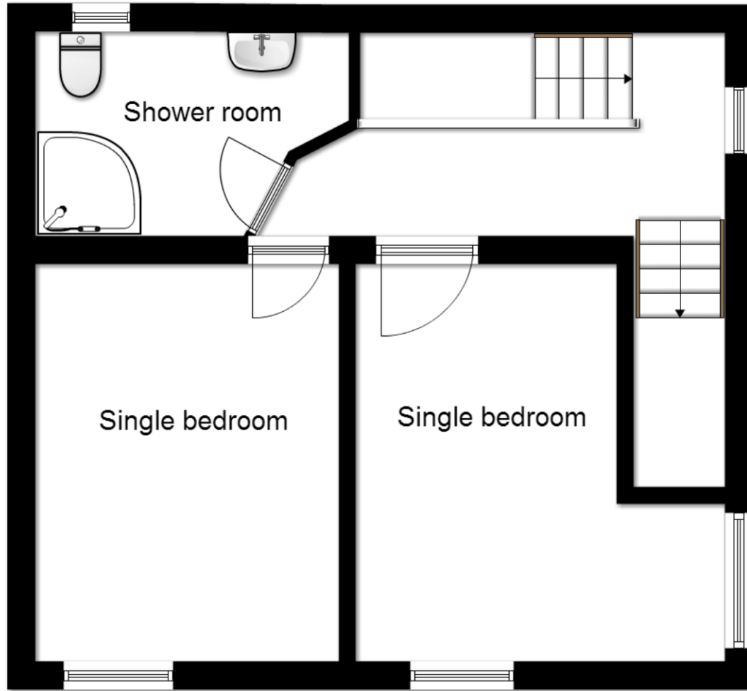
West End Cottage First Floor
